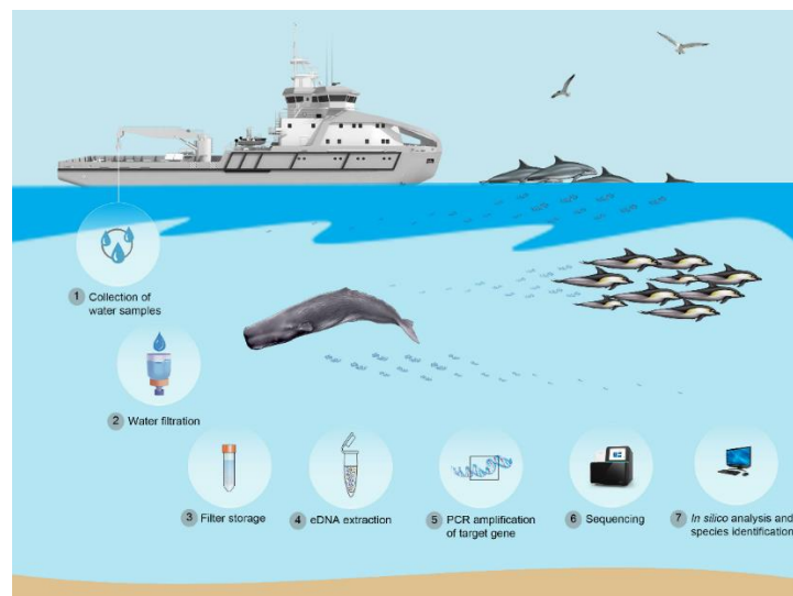
Figure 5. Application of eDNA methodology for marine mammals monitoring (Suarez-Bregua et al., 2022).
